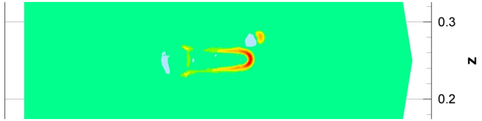
Figure 6.96: Net charge density at times t_1 = 1.31 \cdot 10^{-8} s, isolines in a cut plane y = 0.25
