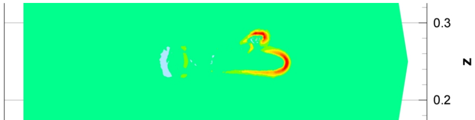
Figure 6.49: Net charge density at times t_1 = 1.47 \cdot 10^{-8} s, isolines in a cut plane y = 0.25
