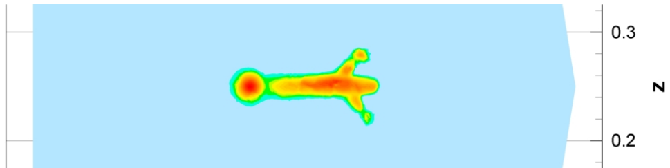
Figure 6.86: Electron density at times t_1 = 1.47 \cdot 10^{-8} s, isolines in a cut plane y = 0.25
