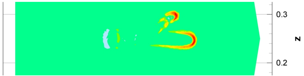
Figure 6.74: Net charge density at times t_1 = 1.68 \cdot 10^{-8} s, isolines in a cut plane y = 0.25
