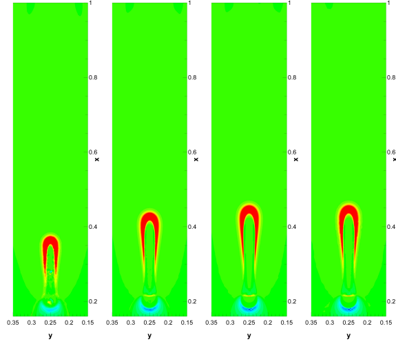
Figure 5.8: 2^{nd} order , comparison of net charge density computed on different uniformly refined meshes at time t = 5.25 \cdot 10^{-8} s . From left to right: 2 levels, 3 levels, 4 levels, adaptation (4 levels)
