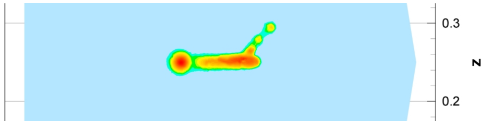
Figure 6.60: Electron density at times t_1 = 1.36 \cdot 10^{-8} s, isolines in a cut plane y = 0.25
