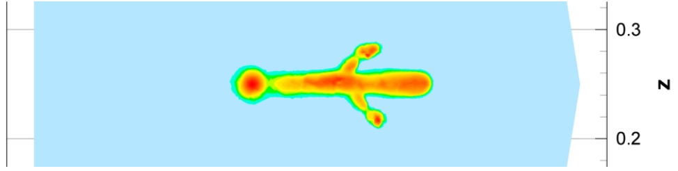
Figure 6.87: Electron density at times t_1 = 1.68 \cdot 10^{-8} s, isolines in a cut plane y = 0.25
