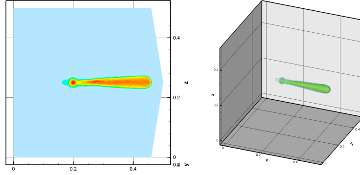
Figure 6.11: Electron density at time t = 1.89 \cdot 10^{-8} s
