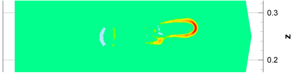
Figure 6.29: Net charge density at times t_1 = 1.68 \cdot 10^{-8} s, isolines in a cut plane y = 0.25
