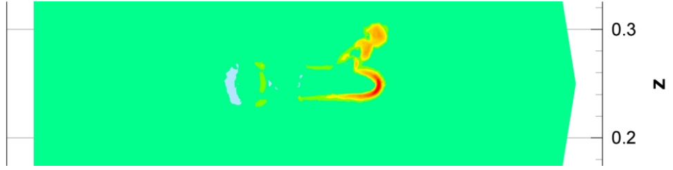
Figure 6.73: Net charge density at times t_1 = 1.47 \cdot 10^{-8} s, isolines in a cut plane y = 0.25
