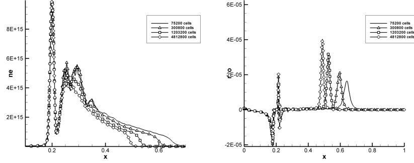
Figure 5.9: 1^{st} order, comparison of electron density (left) and net charge density (right) computed on different coarse meshes at time t = 5.25 \cdot 10^{-8} s : 2 levels, 3 levels, 4 levels, 5 levels
