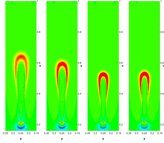
Figure 5.7: 1^{st} order , comparison of net charge density computed on different uniformly refined meshes at time t = 5.25 \cdot 10^{-8} s . From left to right: 2 levels, 3 levels, 4 levels, adaptation (4 levels)
