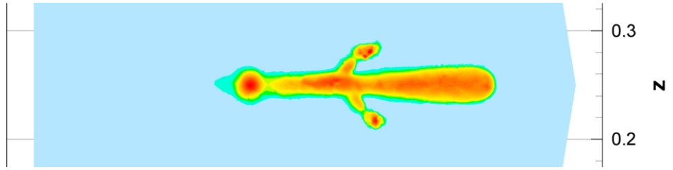
Figure 6.88: Electron density at times t_1 = 1.89 \cdot 10^{-8} s, isolines in a cut plane y = 0.25
