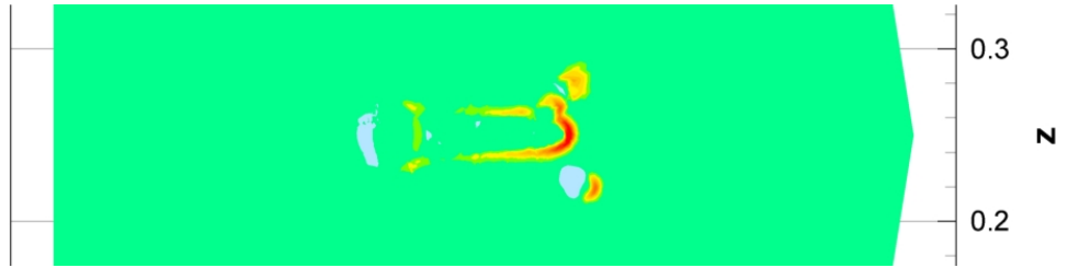
Figure 6.97: Net charge density at times t_1 = 1.36 \cdot 10^{-8} s, isolines in a cut plane y = 0.25
