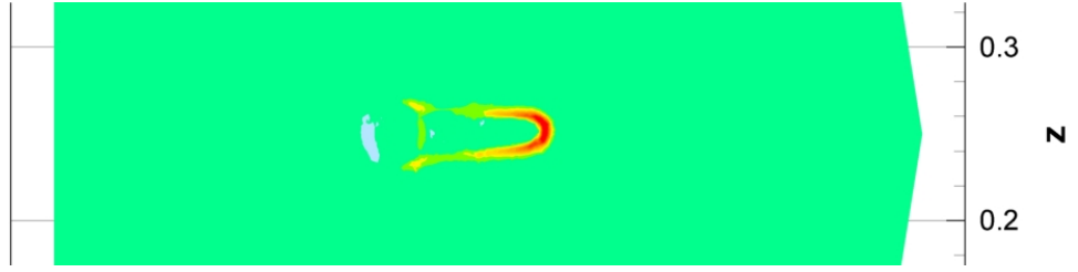
Figure 6.95: Net charge density at times t_1 = 1.26 \cdot 10^{-8} s, isolines in a cut plane y = 0.25
