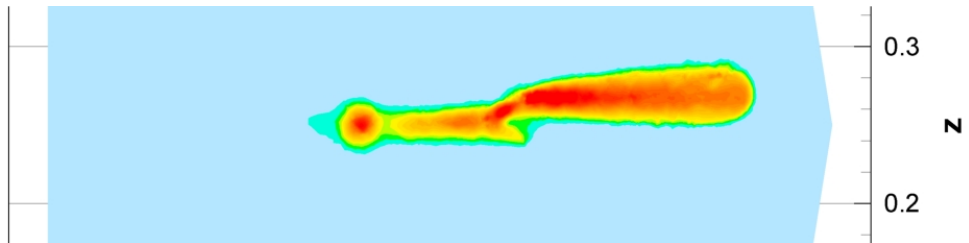
Figure 6.20: Electron density at times t_1 = 1.89 \cdot 10^{-8} s, isolines in a cut plane y = 0.25
